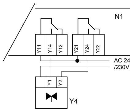
Optional 3-position control (appl. A1, A2 & A8)
