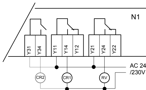
Heat pumps (appl. A5)
