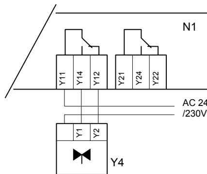
2-pipe FCU, 2-position control (appl. A8)
