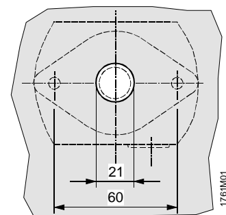
Drilling plan
